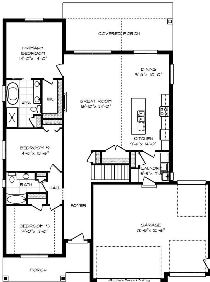
MAIN FLOOR 1922 SQ. FT. 52'-0" HOUSE WIDTH
