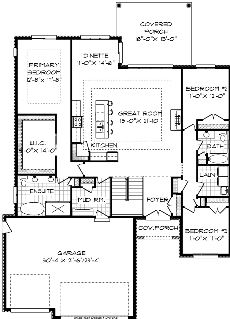
MAIN FLOOR 2188 SQ. FT. 54'-8" HOUSE WIDTH
