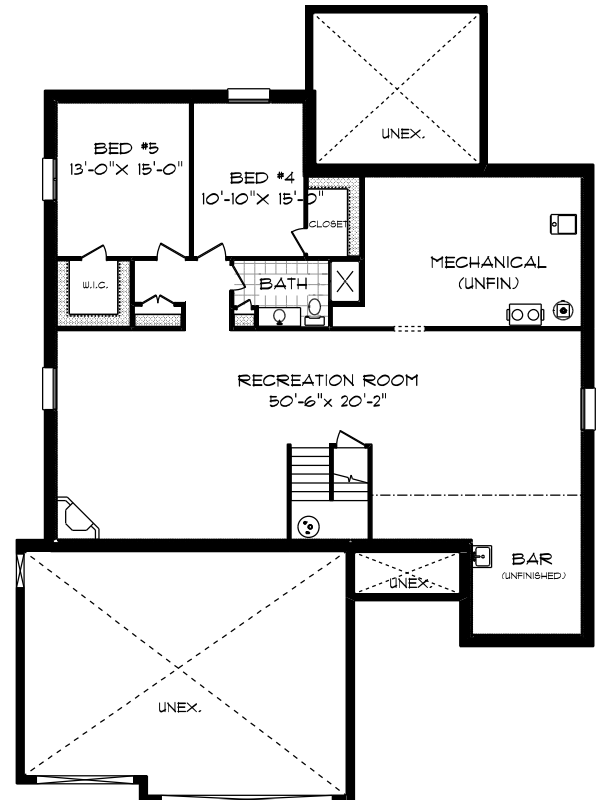
BASEMENT 1572 SQ. FT. (FIN)
